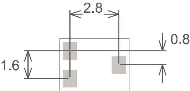
Pads 1-3 = 1.0 x 0.8 (mm)
